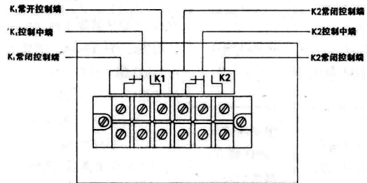
XWBJ-101, XQBJ-101 型 XWBJ-102, XQBJ-102 型 XWBJ-108, XQBJ-108 型 (二接点) XWBJ-121, XQBJ-121 型
